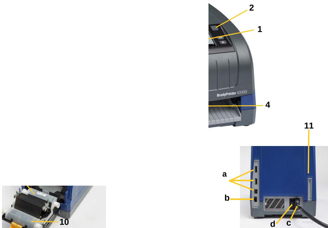
Figure 2-1. Printer Components
