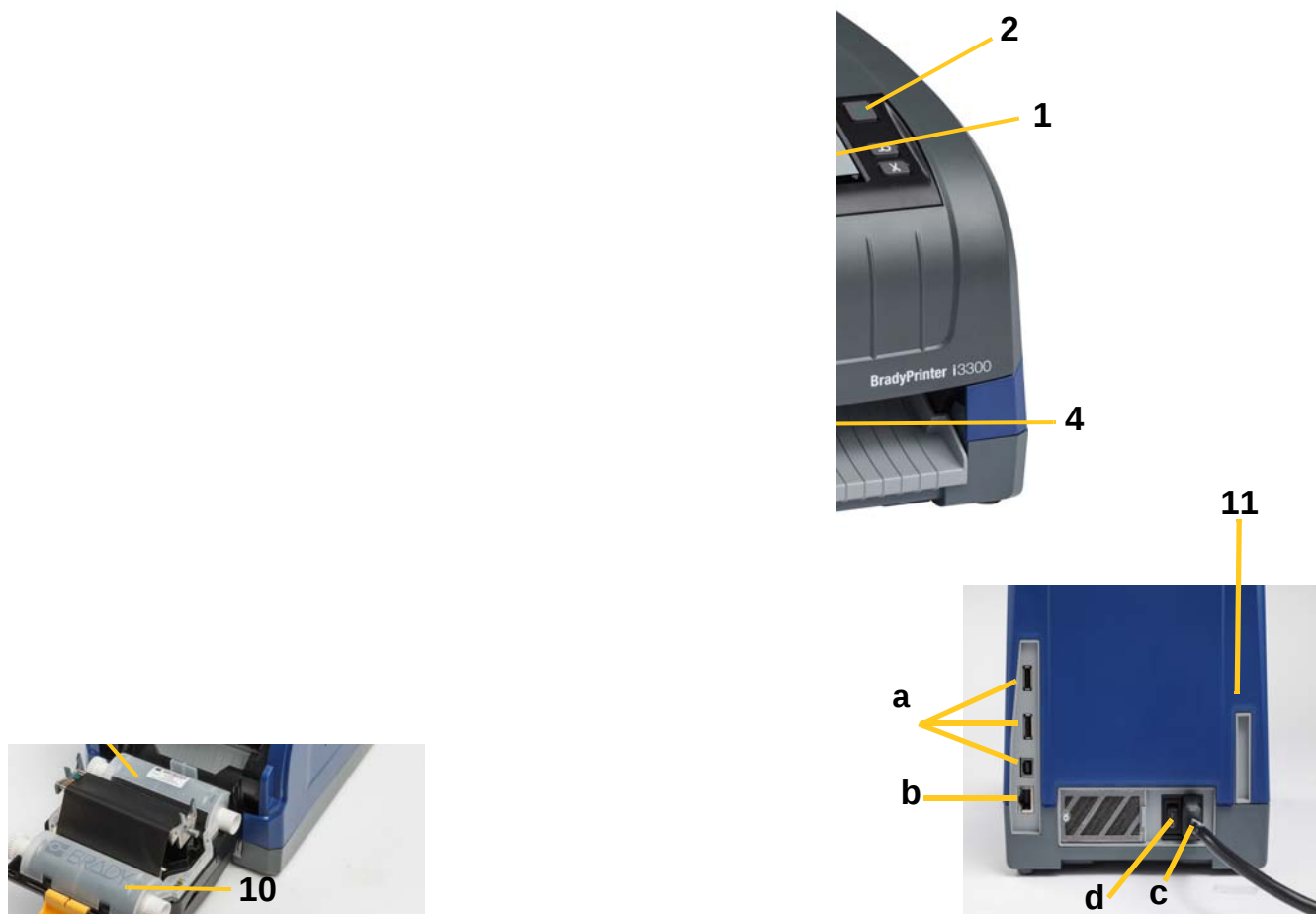
Figure 2-1. Printer Components
